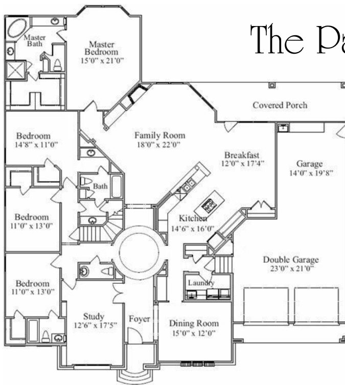
Floor Plan
